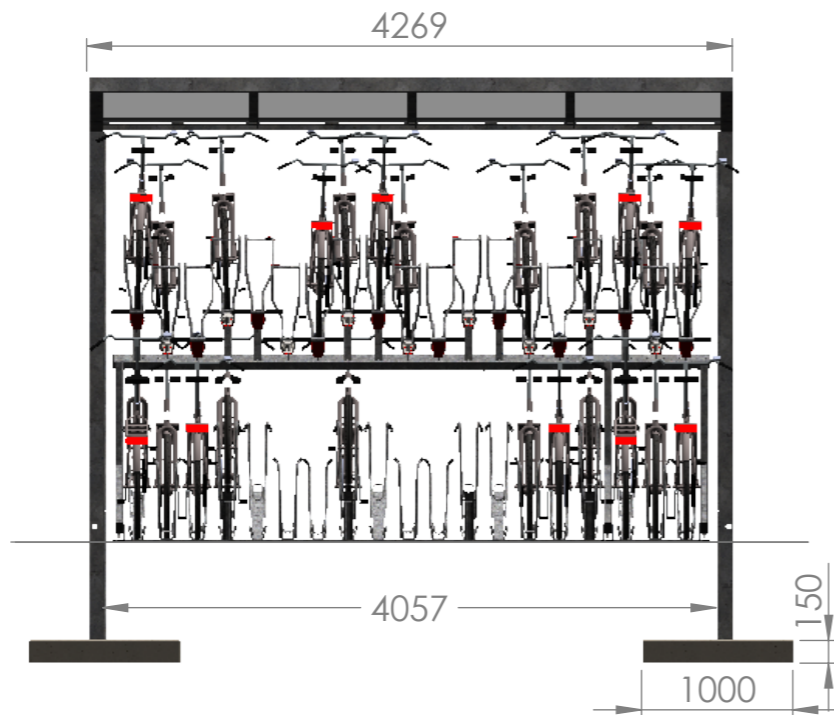
T-Hide Up double-sided 1 section - h.2.h. 400 mm
