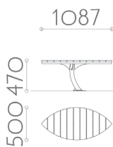
1 seat Ref. 17 0501 ED10 AE00 1087 x 500 x HT 470 mm Weight: 23 kg
