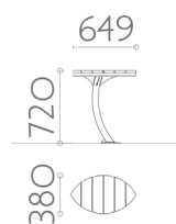
1 shelf Ref. 17 0510 ED10 AE00 688 x 380 x HT 720 mm Weight: 16 kg
