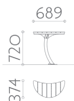
1 curve shelf Ref. 17 0515 ED10 AE00 688 x 380 x HT 720 mm Weight: 16 kg
