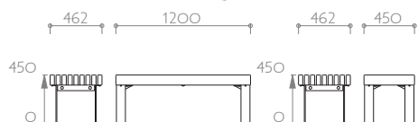
2 place slim bench
