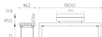
3 place bench half backrest
