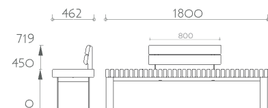
3 place seat half-backrest
